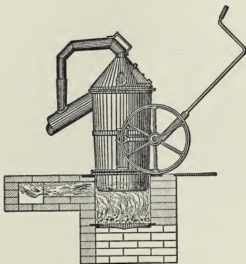
FIG. 18.—Sommer's Kettle, Truck, and Fire.
